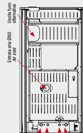
Mandata impianto 3/4" System entrance 3/4" Calda sanitaria 1/2" Hot sanitary 1/2" Ritorno impianto 3/4" System return 3/4" Fredda sanitaria 1/2" Cold sanitary 1/2"
